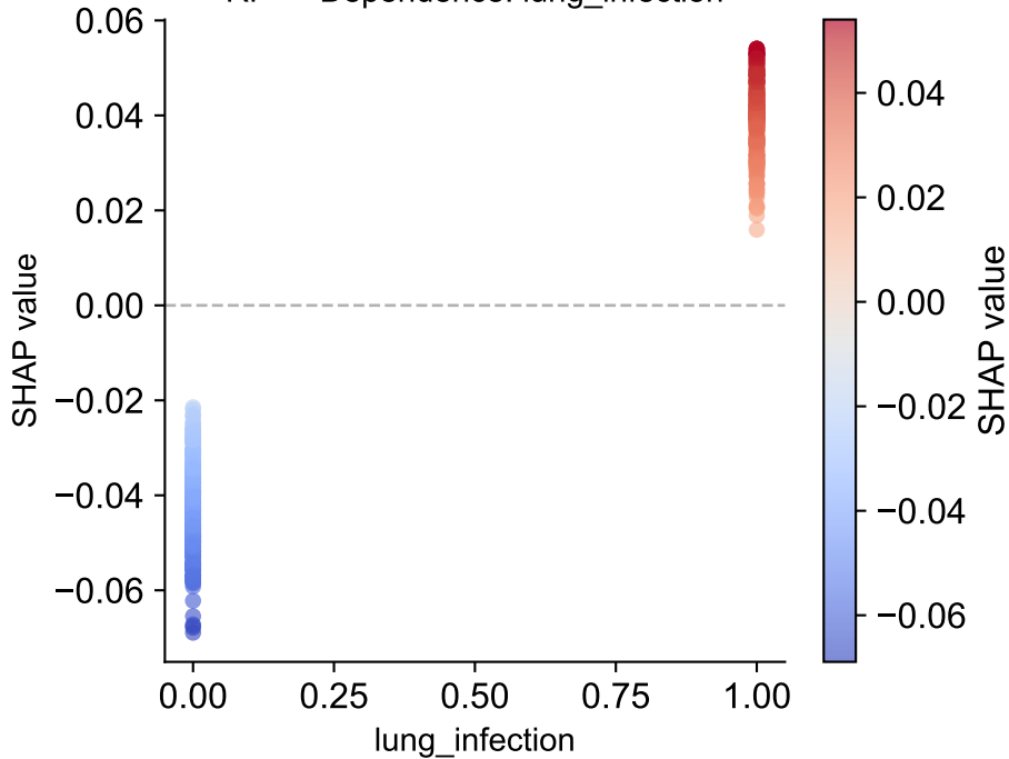
RF — Dependence: lung_infection
