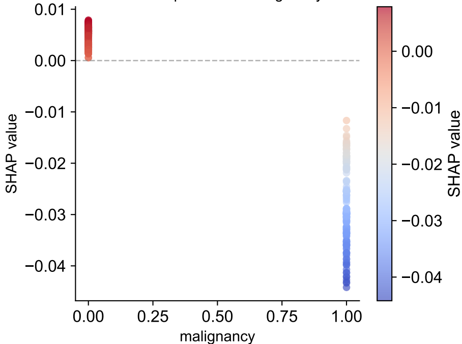
RF — Dependence: malignancy
