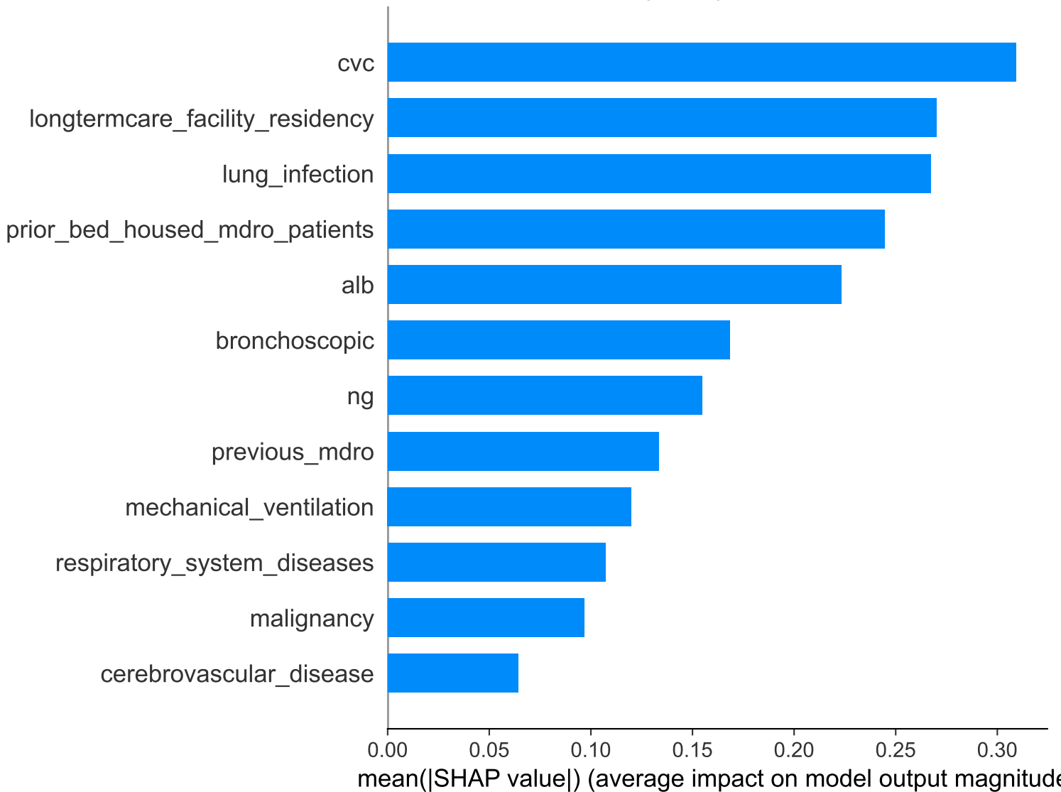
XGB — Mean |SHAP| Feature Importance
