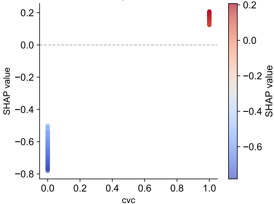
XGB — Dependence: cvc
