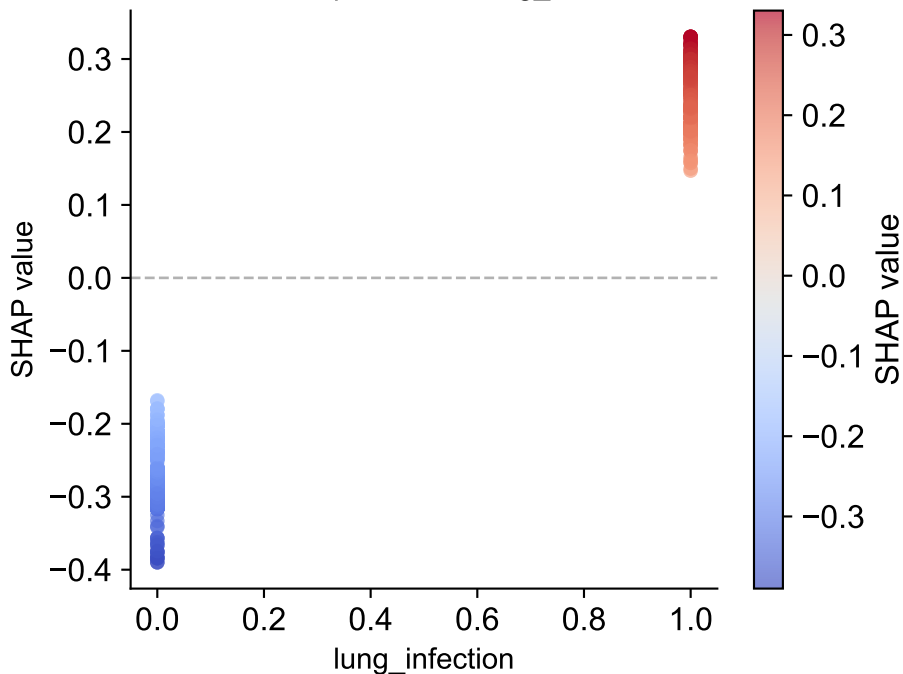
XGB — Dependence: lung_infection
