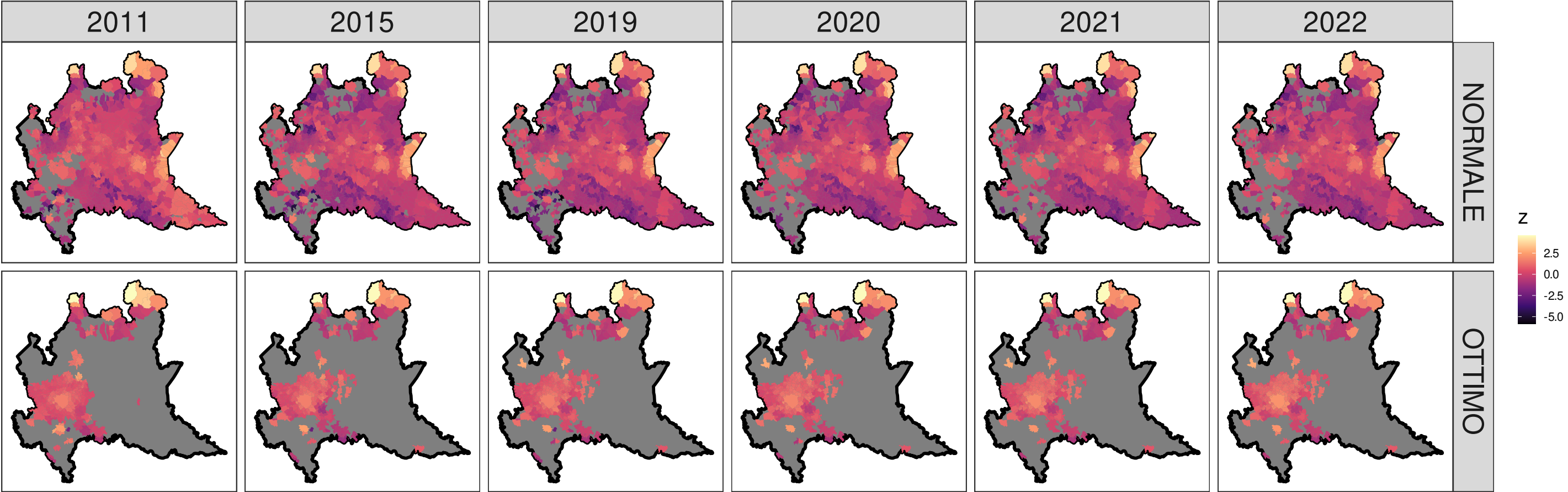
Log prices for Rents of 'Uffici' (normalized)
