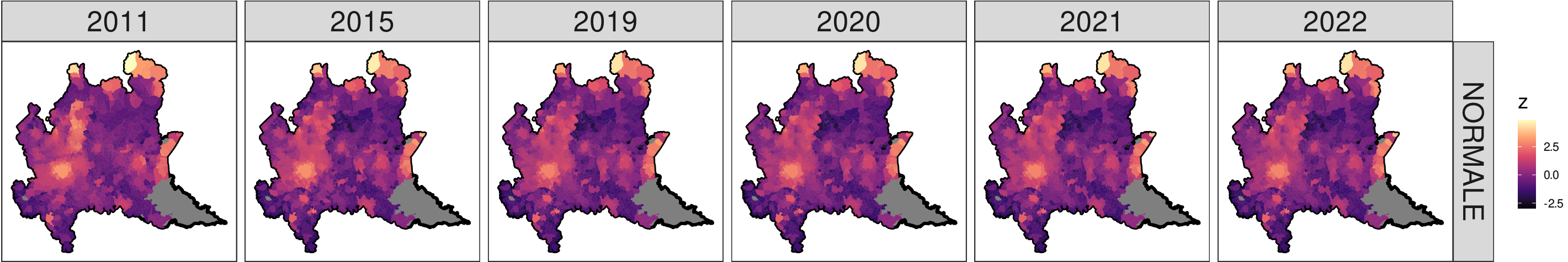
Log prices for Sales of 'Box' (normalized)
