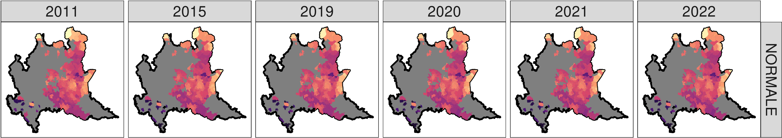
Log prices for Sales of 'Posti_auto_scoperti' (normalized)
