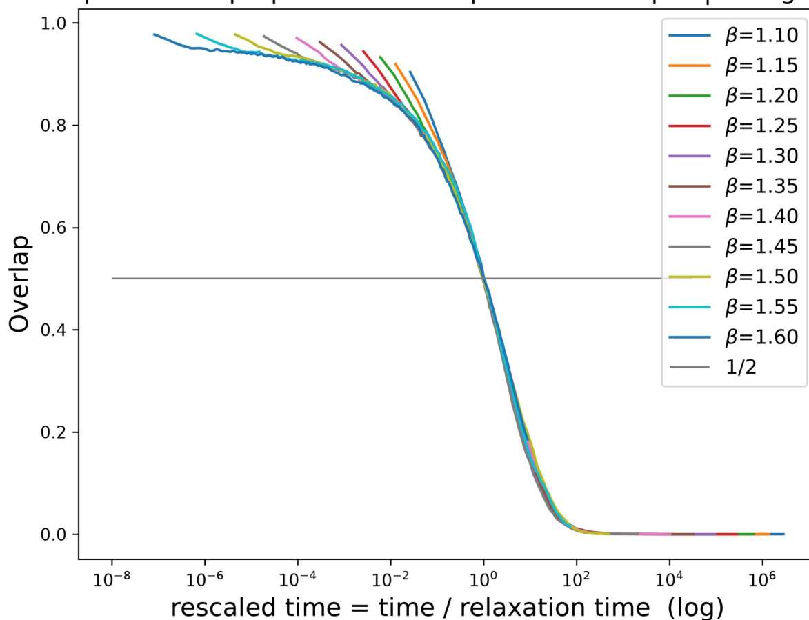
Time-temperature superposition: Overlap curves' collapse | Triangular lattice
