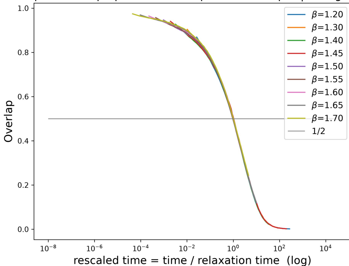
Time-temperature superposition: Overlap curves' collapse | Hexagonal lattice
