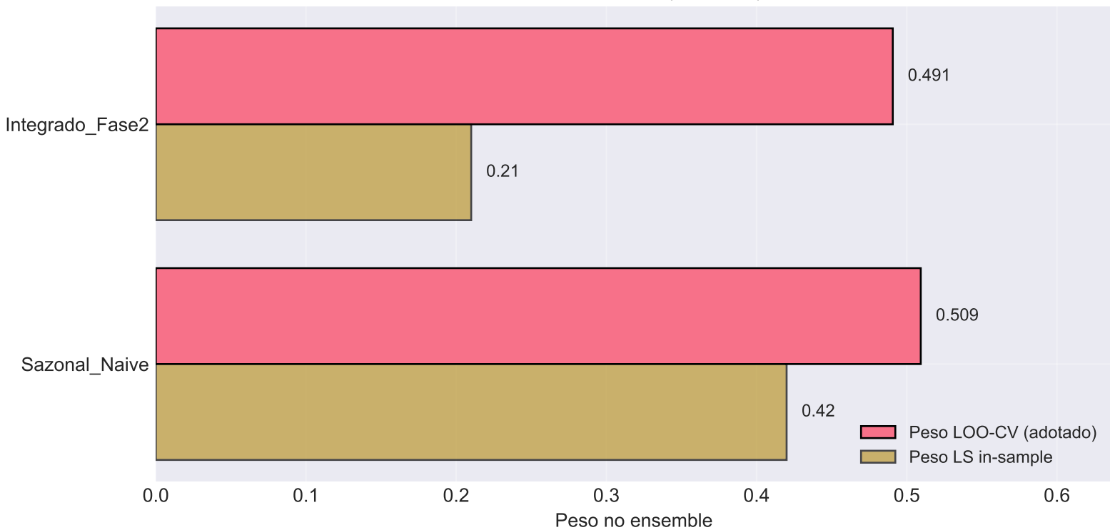
Pesos do ensemble — LOO-CV (adotado) vs LS in-sample
