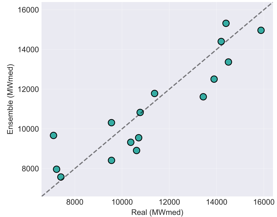
Scatter Real x Ensemble (r=0.904)
