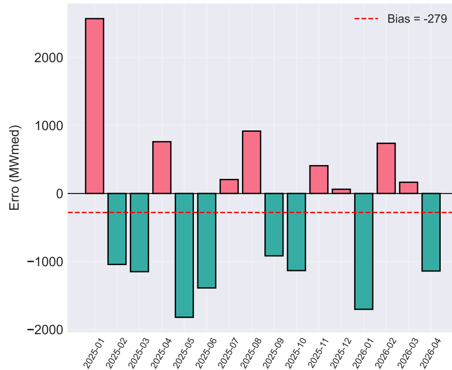
Residuos Ensemble - Real
