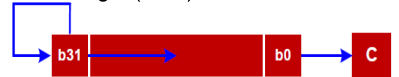
Arithmetic Shift Right ( ASR )
