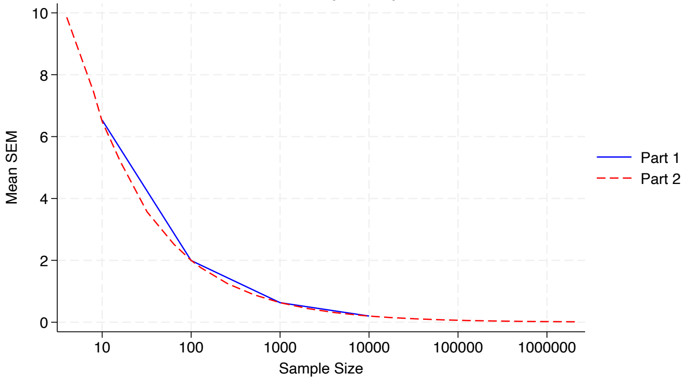
Standard Error by Sample Size
