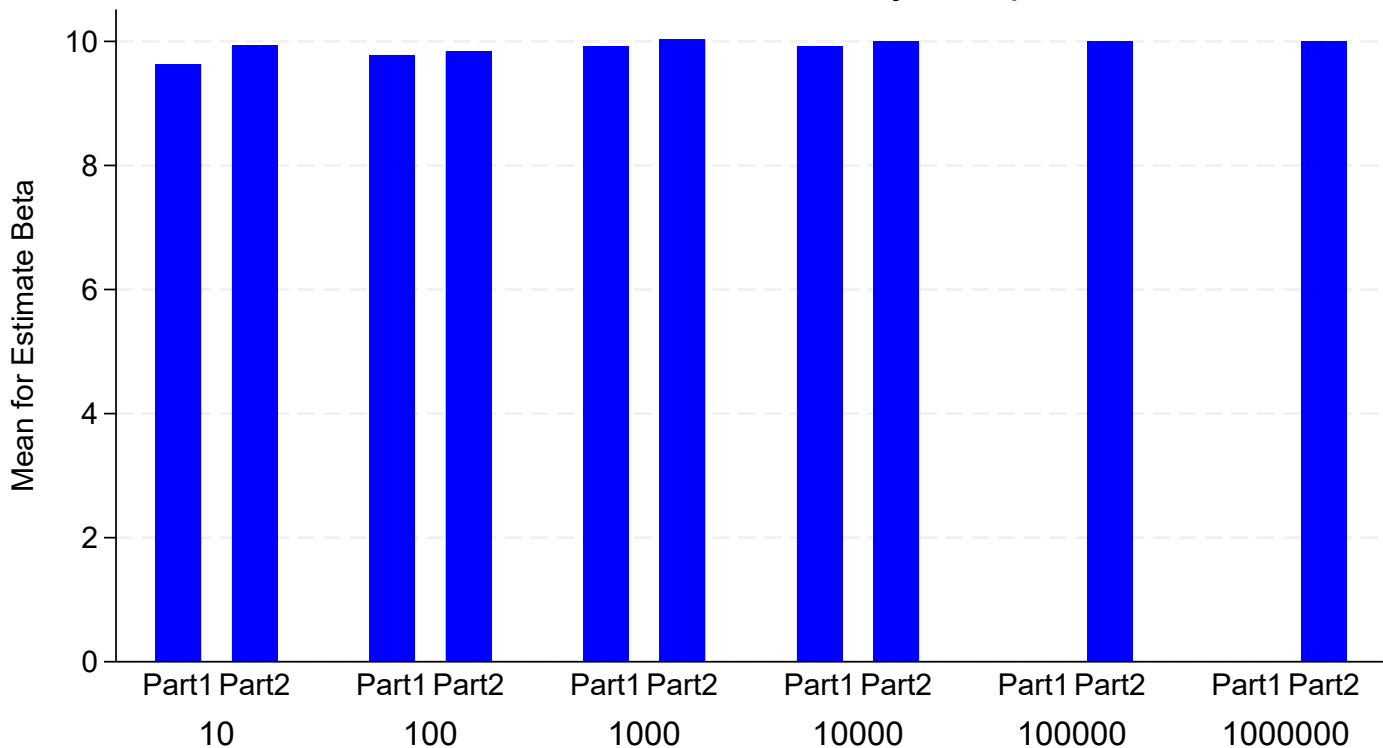
Mean Estimates of Beta for Key Sample Sizes
