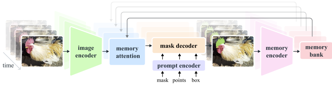
Figure 3.7. Architecture de SAM-2 (figure issue de [39]).
