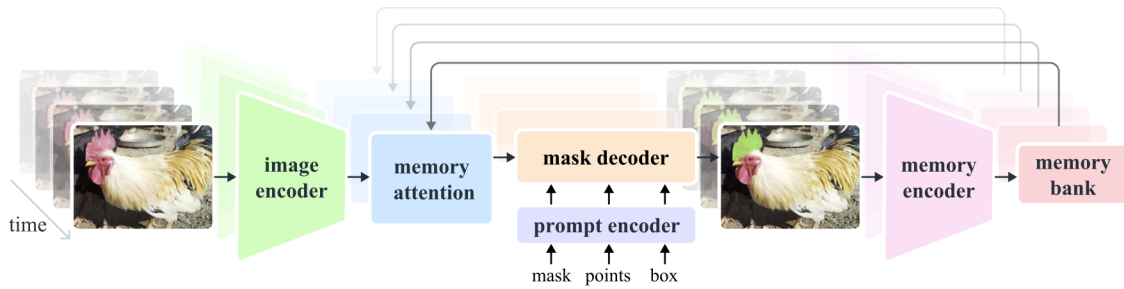
Figure 4.1. Architecture de SAM-2 (figure issue de [3]).
