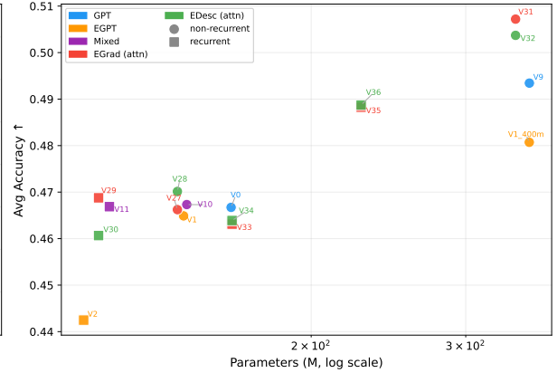
Figure 15: Clean PPL and accuracy vs. parameters (same as Figs. 1, 2 in main text). Mixed mislabeled runs excluded.
