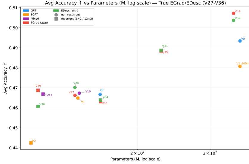
Figure 10: EGrad(attn)/EDesc(attn) (V27–V36) vs. baselines: accuracy vs. parameters. EGrad (red) and EDesc (green) cluster tightly with MixedHead (purple), confirming the output rule provides no additional gain over the mixed-head baseline at 144M scale. See Appendix E for full scatter plots.
