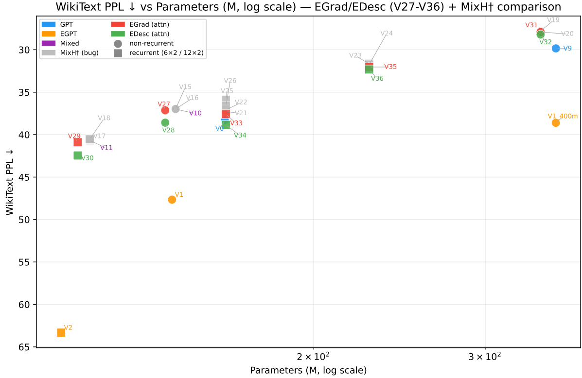
Figure 16: PPL vs. parameters — all runs including Mixed (grey). Grey points (V15–V26) are mislabeled: intended as EGrad/EDesc but trained as plain MixedHead due to a config serialization bug (see §2). Shown here for reference only; not used in any main-text figures or conclusions.
