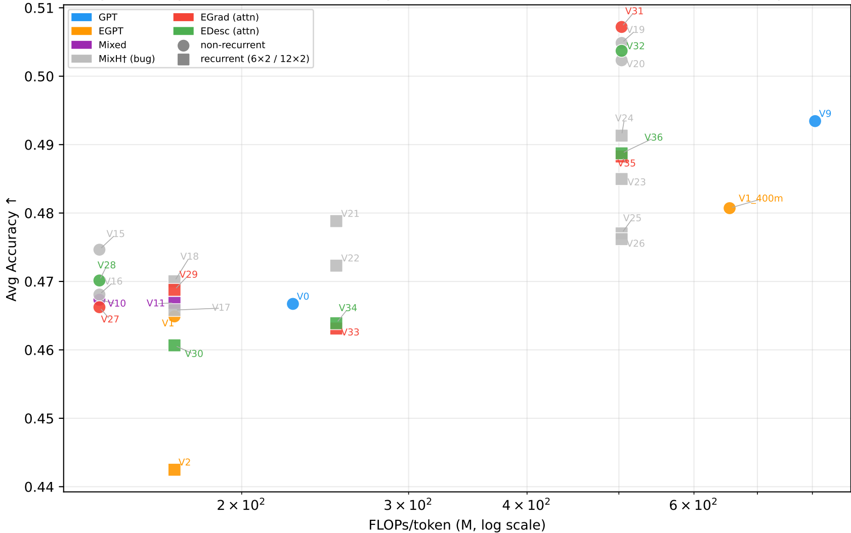
Avg Accuracy ↑ vs FLOPs/token (M, log scale) — EGrad/EDesc (V27-V36) + MixH† comparison
