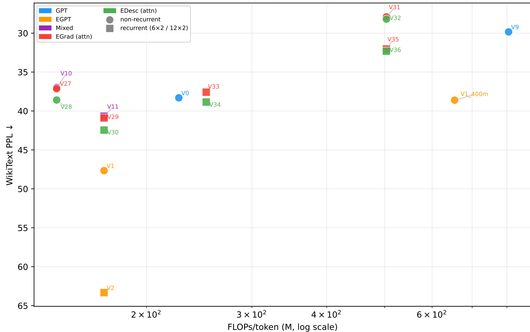
WikiText PPL ↓ vs FLOPs/token (M, log scale) — True EGrad/EDesc (V27-V36)
