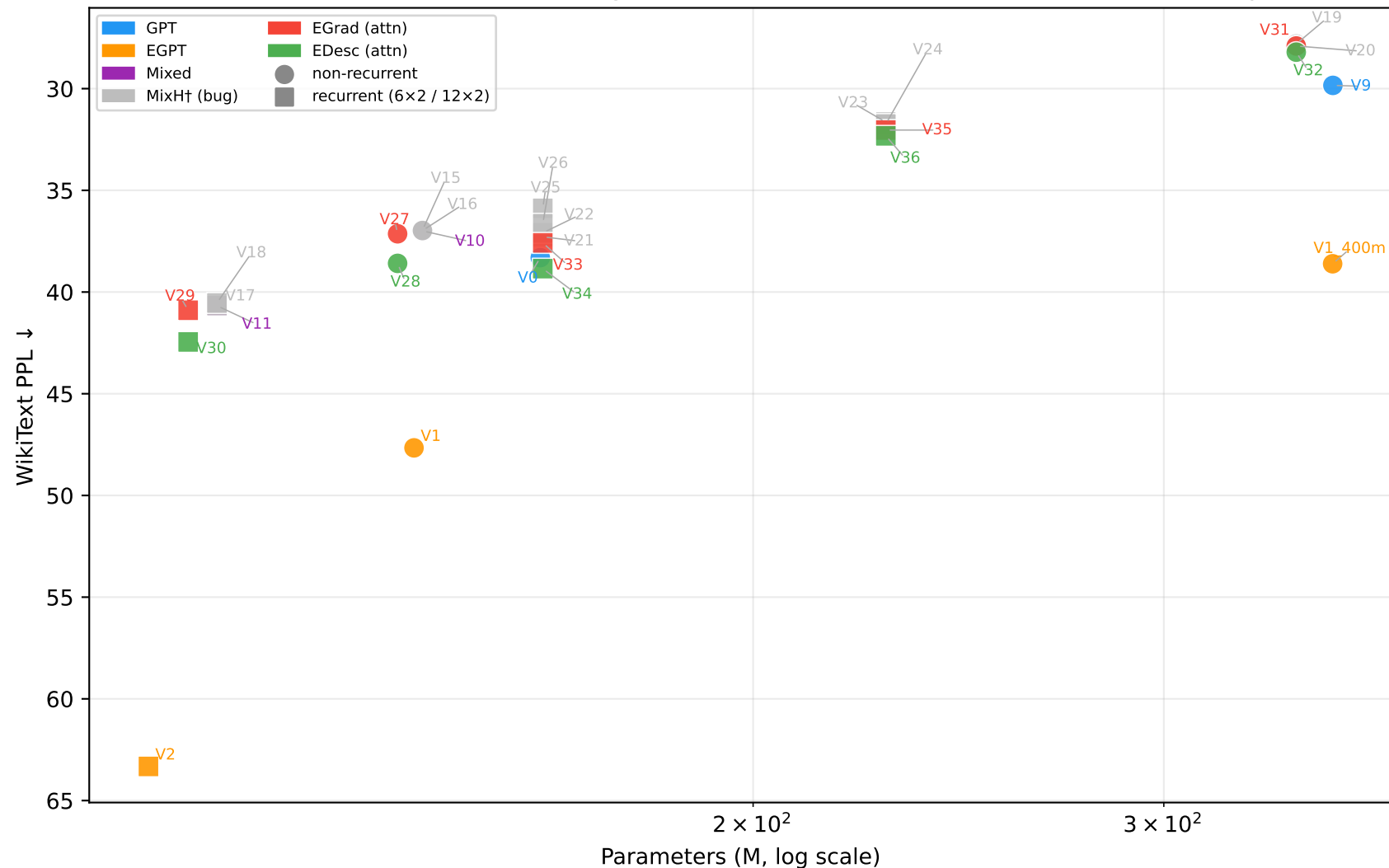
WikiText PPL ↓ vs Parameters (M, log scale) — EGrad/EDesc (V27-V36) + MixH† comparison
