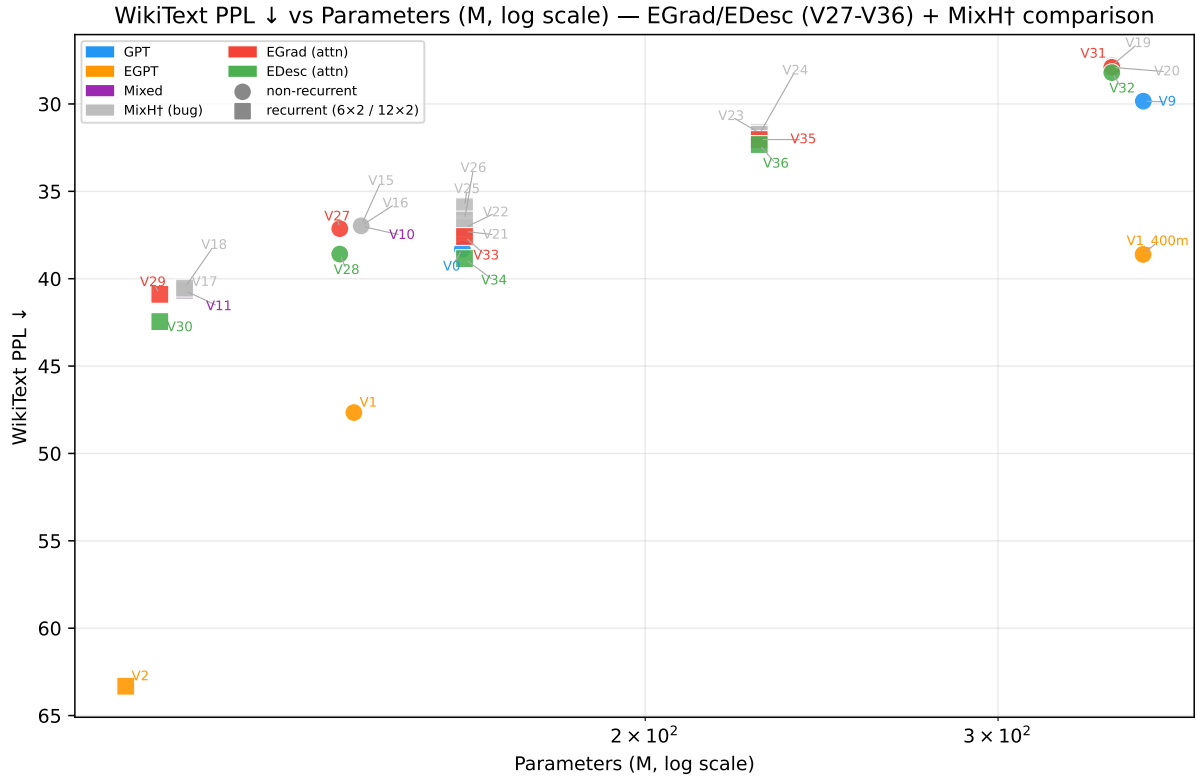
Figure 37: PPL vs. parameters — all runs including Mixed (grey). Grey points (V15–V26) are mislabeled: intended as EGrad/EDesc but trained as plain MixedHead due to a config serialization bug (see §2). Shown here for reference only; not used in any main-text figures or conclusions.
