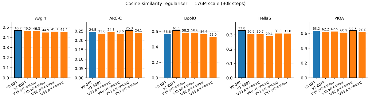
Figure 6: Cosine-similarity regulariser benchmark performance (176M, 30k steps, 30k \times 4 \text{ GPU} \times 7.86\text{B} tokens). Light cosreg ( \lambda=0.01 , V39 act / V48 wt) is roughly free; the stronger variants V52 ( \lambda=0.1 ) and V53 (cosine ramp 0 \rightarrow 1.0 ) cost \approx 0.8 – 1.1 accuracy points on average vs V1 EGPT, while V53’s WikiPPL (47.7) is identical to V1’s — strong cosreg does not hurt perplexity. V48 (weight-cosreg) loses the most ( -1.6 acc, +14.9 PPL vs V1). See §2.7 for FLOPs and training-time analysis.
