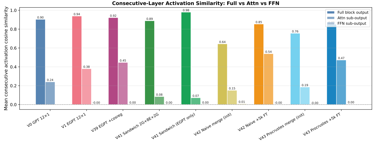
Figure 31: Consecutive-layer activation cosine similarity breakdown: residual stream, attn sub-output, FFN sub-output. V41 EGPT-only entry shows consecutive similarity for EGPT-EGPT layer pairs only.
