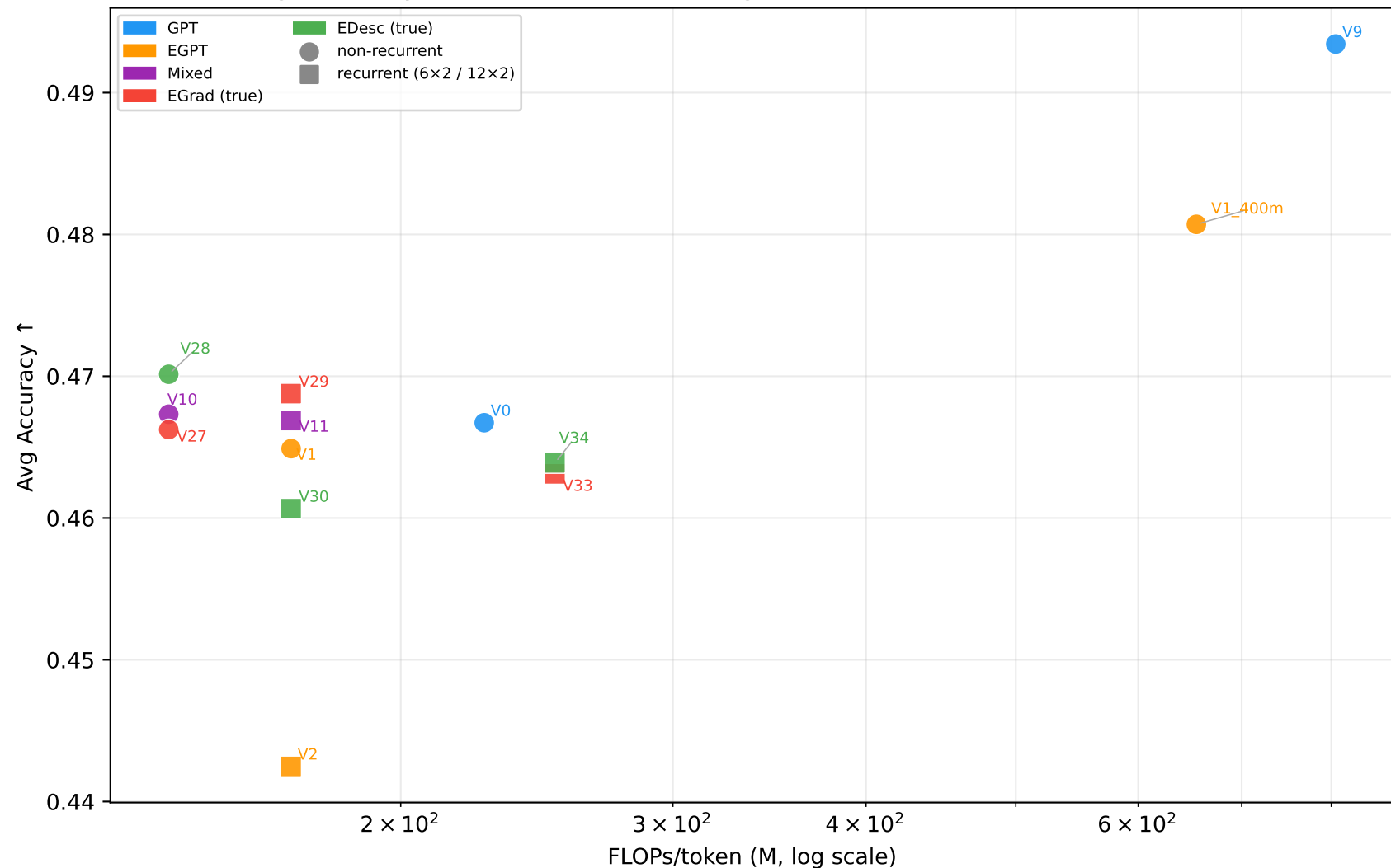
Avg Accuracy ↑ vs FLOPs/token (M, log scale) — True EGrad/EDesc (V27-V36)
