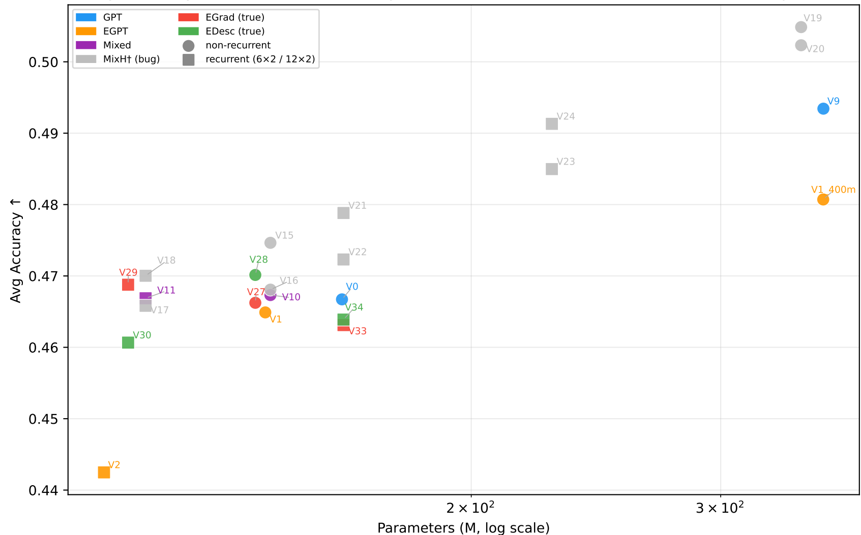
Avg Accuracy ↑ vs Parameters (M, log scale) — EGrad/EDesc (V27-V36) + MixH† comparison
