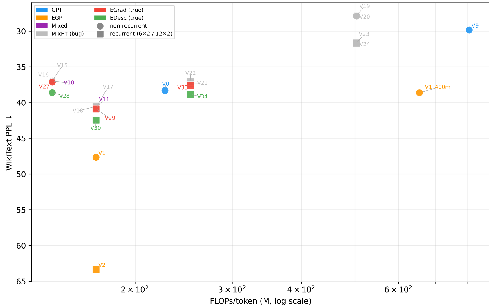
WikiText PPL ↓ vs FLOPs/token (M, log scale) — EGrad/EDesc (V27-V36) + MixH† comparison
