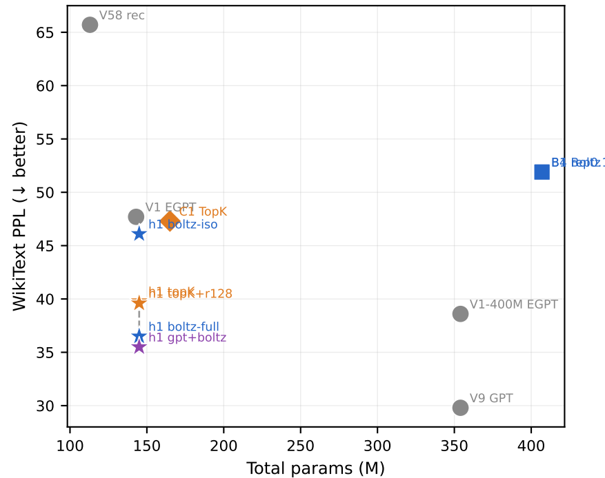
MoE variants vs baselines (7.86B tokens, same architecture family)
