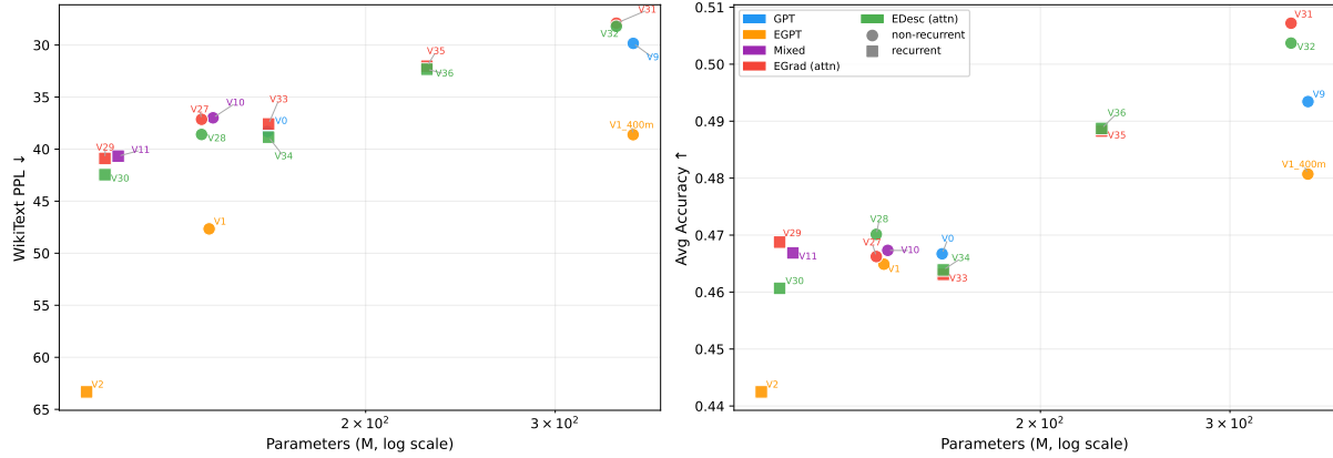
Figure 36: Clean PPL and accuracy vs. parameters (same as Figs. 1, 2 in main text). Mixed mislabeled runs excluded.
