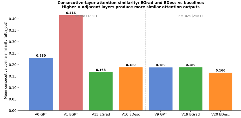
Figure 13: Consecutive-layer mean attn_out cosine similarity (adjacent pairs only). Same trend as the off-diagonal mean: V1 EGPT has highest consecutive alignment.
