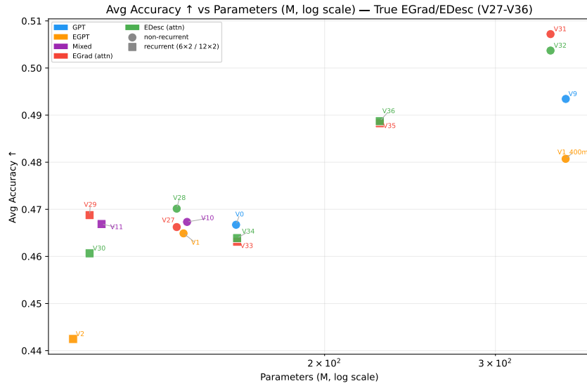
Figure 15: EGrad(attn)/EDesc(attn) (V27–V36) vs. baselines: accuracy vs. parameters. EGrad (red) and EDesc (green) cluster tightly with MixedHead (purple), confirming the output rule provides no additional gain over the mixed-head baseline at 144M scale. See Appendix E for full scatter plots.
