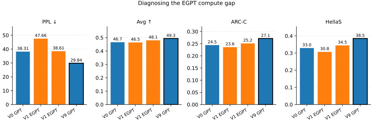
Figure 3: Diagnosing the EGPT compute gap. Bars compare V0 GPT 12×1 (162M, 321 MFLOPs/tok), V1 EGPT 12×1 (143M, 359 MFLOPs/tok), V1 EGPT 24×1 (400M, 755 MFLOPs/tok), and V9 GPT 24×1 (354M, 503 MFLOPs/tok). EGPT trails GPT on PPL despite higher FLOPs.
