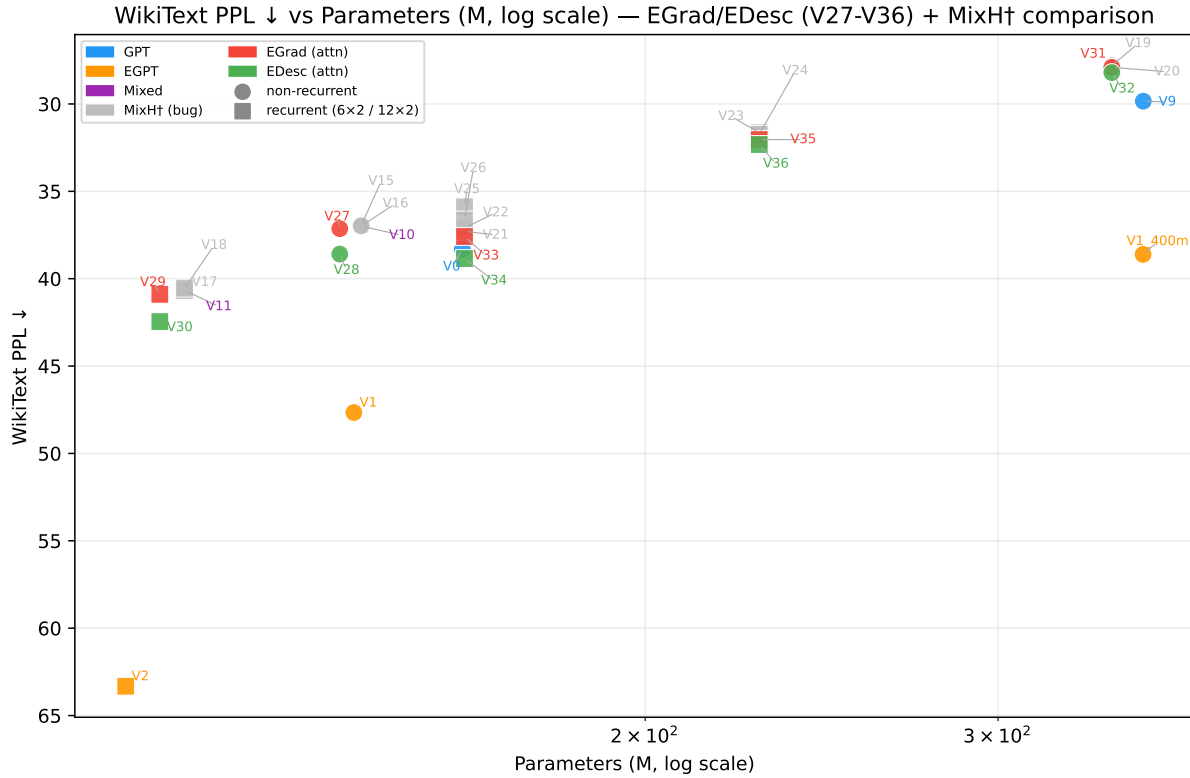
Figure 37: PPL vs. parameters — all runs including Mixed (grey). Grey points (V15–V26) are mislabeled: intended as EGrad/EDesc but trained as plain MixedHead due to a config serialization bug (see §2). Shown here for reference only; not used in any main-text figures or conclusions.
