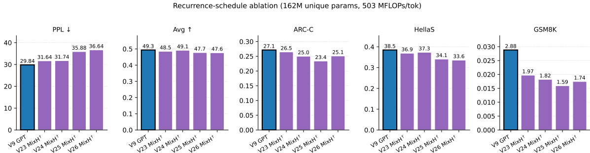
Figure 5: Recurrence-schedule ablation (Mixed, 162M unique params, 503 MFLOPs/token, 30k steps). V25 (uniform 6×4) and V26 (back-loaded 6×ramp) test whether more or non-uniform recurrence beats V23/V24 12×2.
