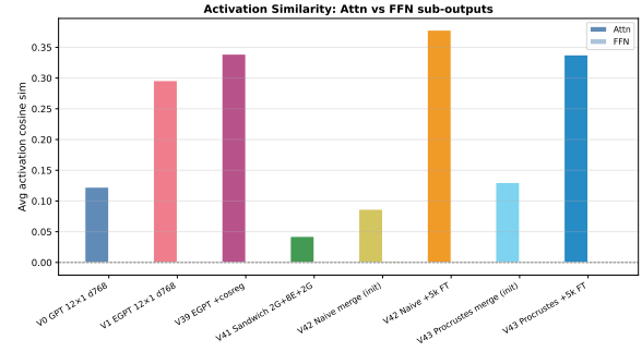
Figure 28: Attn vs. FFN breakdown of off-diagonal mean activation cosine similarity.
