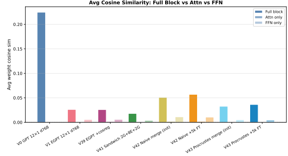
Figure 23: Attn vs. FFN breakdown of off-diagonal mean cosine similarity.
