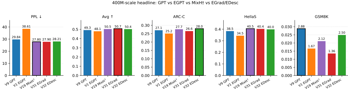
Figure 4: 400M-scale headline. V19 MixHt † , V31 EGrad, and V32 EDesc dominate the V9 GPT baseline on Avg accuracy and PPL at matched compute (503 MFLOPs/token); V1 EGPT 24×1 trails despite using more FLOPs.
