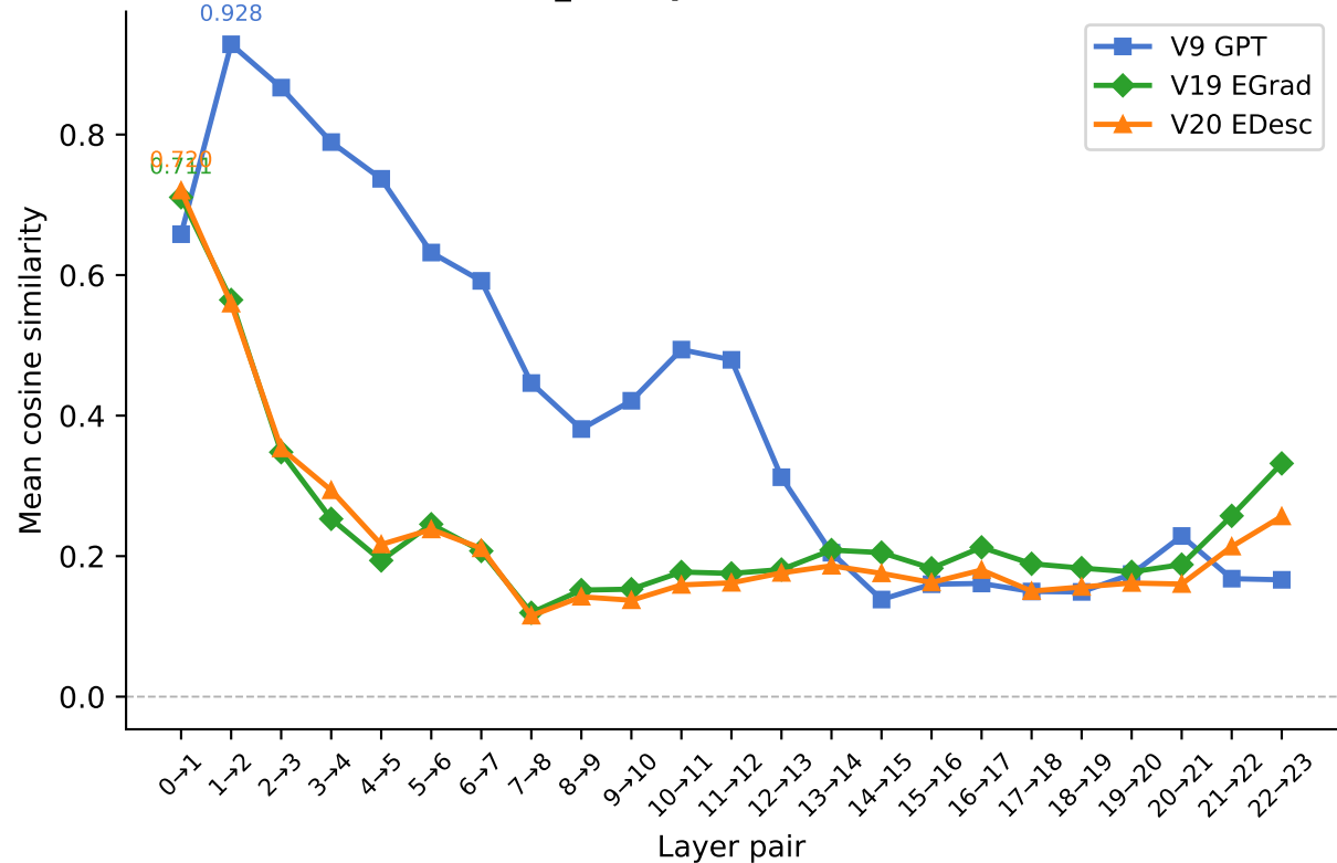
ffwd_out (pre-residual FFN)
