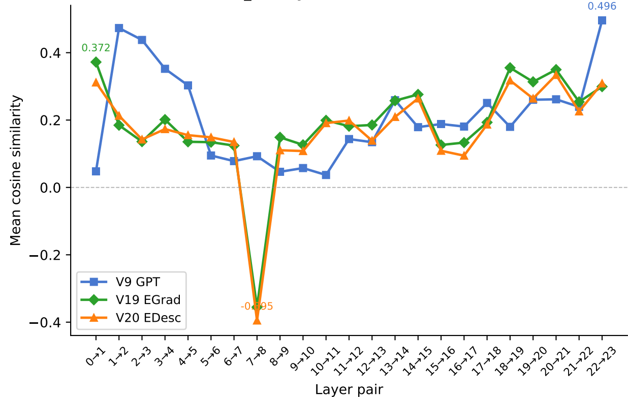
attn_out (pre-residual attention)
