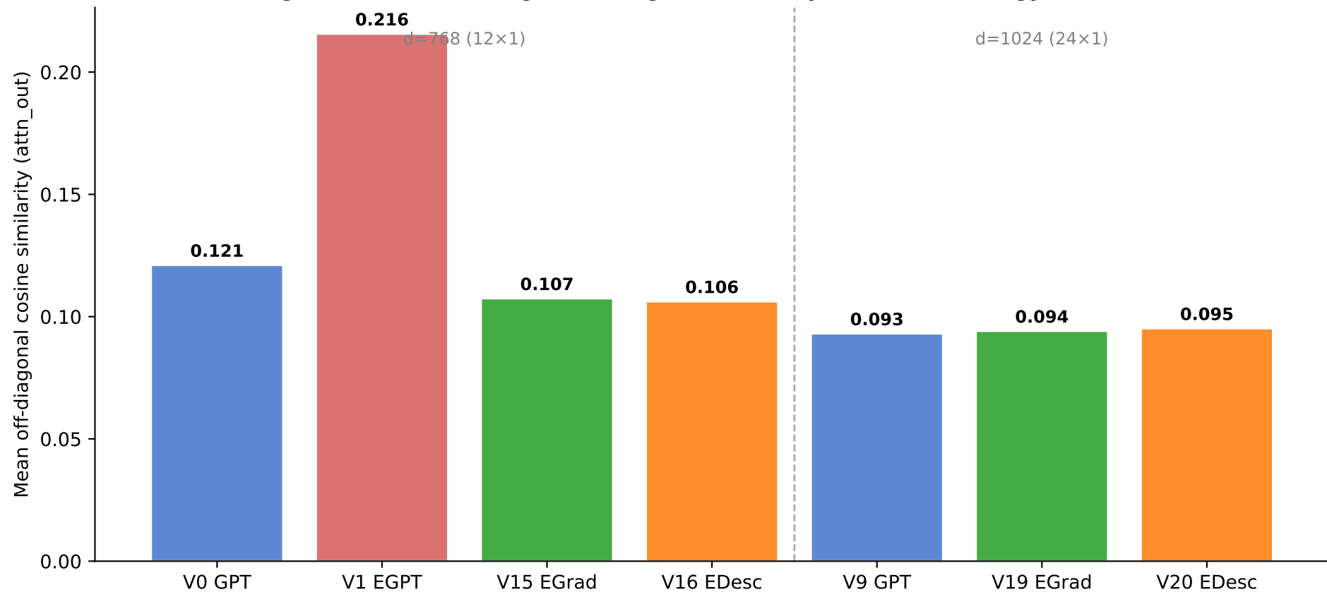
Inter-layer attention similarity: EGrad and EDesc vs baselines Higher = more similar gradient signal across layers (shared energy structure)
