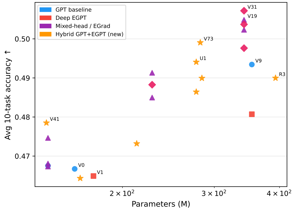
Accuracy vs. Parameters
