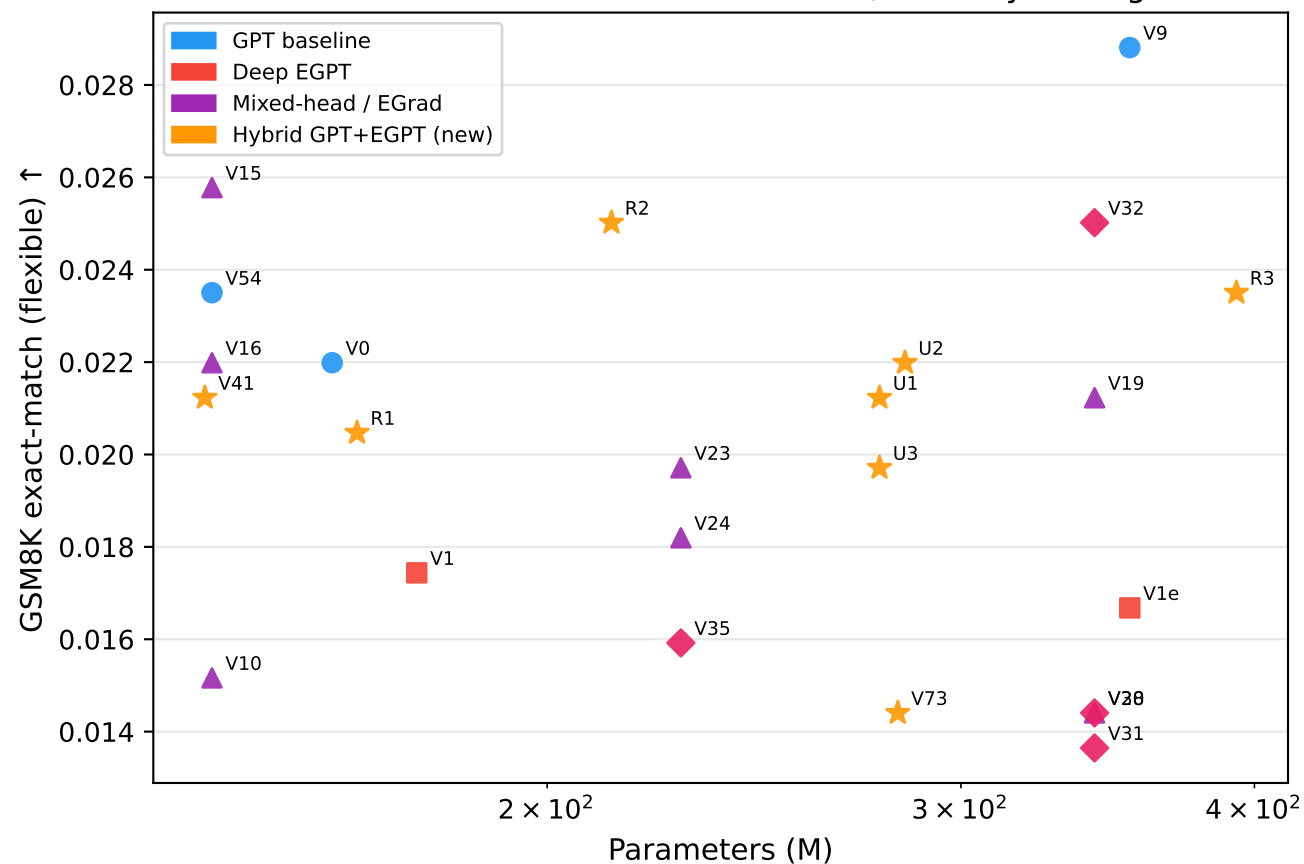
GSM8K vs. Parameters — GPT leads; EGPT/hybrid lag
