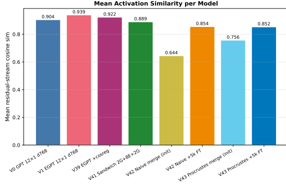
Figure 27: Consecutive-layer mean residual-stream cosine similarity per model (already consecutive, not off-diagonal).
