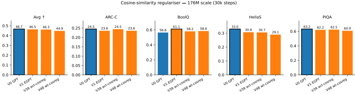
Figure 6: Cosine-similarity regulariser performance (176M, 30k steps). V39 act-cosreg and V48 wt-cosreg ( \lambda=0.01 ) impose minimal accuracy overhead vs V0 GPT and V1 EGPT.
