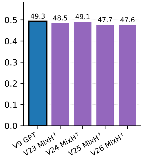
Avg ↑
