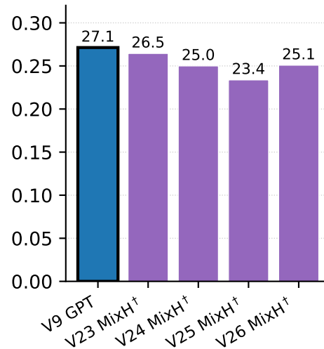
ARC-C
