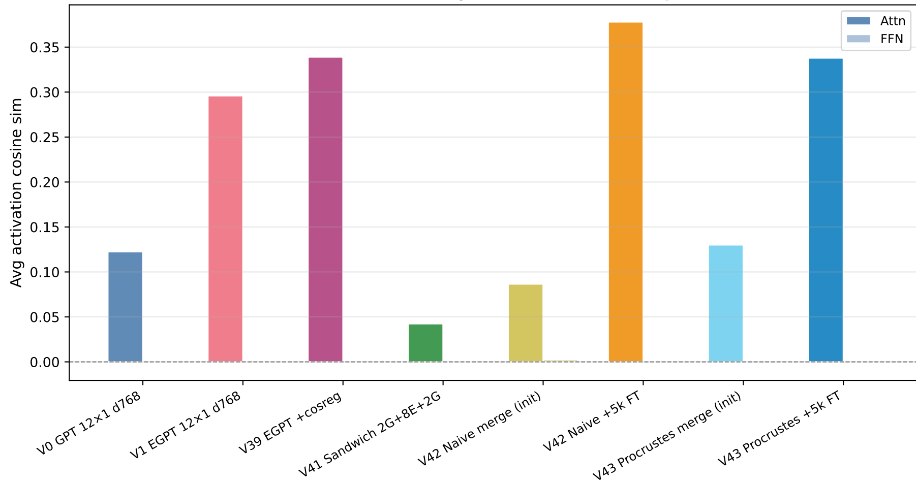
Activation Similarity: Attn vs FFN sub-outputs
