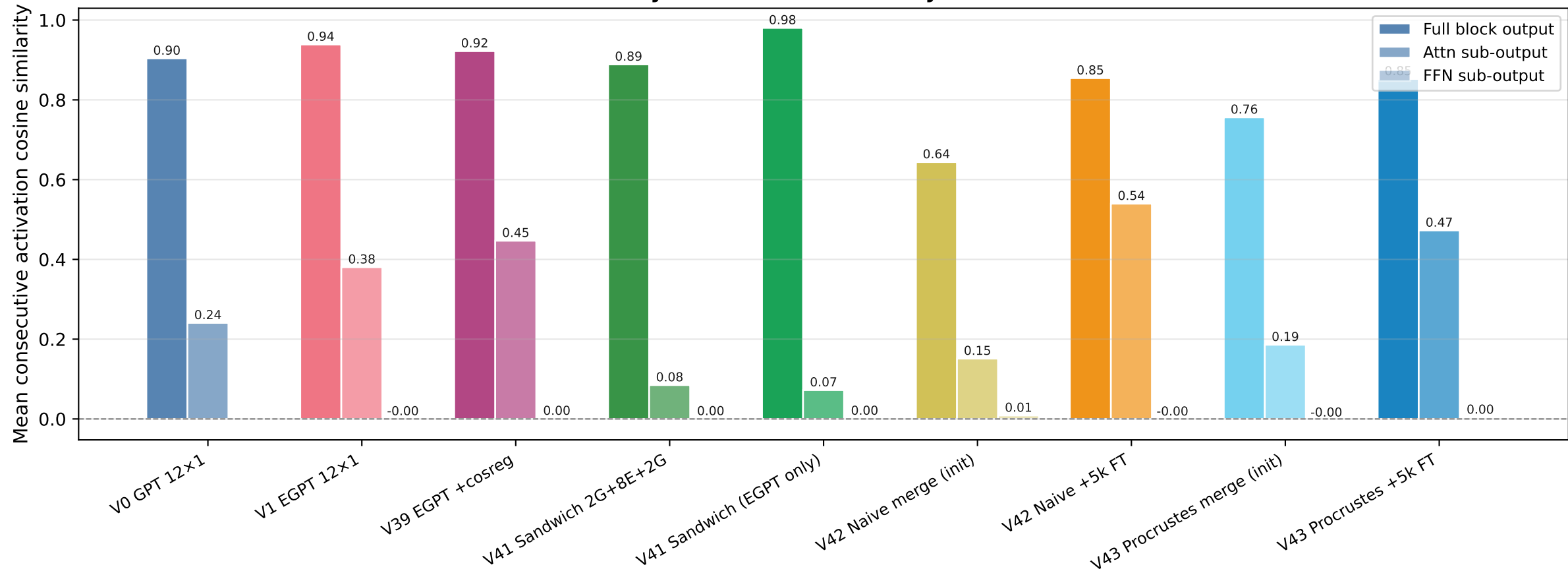
Consecutive-Layer Activation Similarity: Full vs Attn vs FFN
