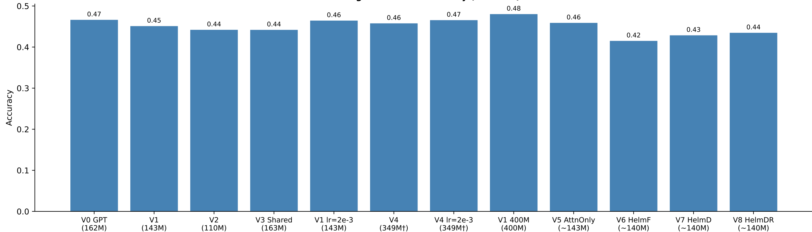
Average Zero-Shot Accuracy (10 tasks)
