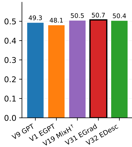
Avg ↑
