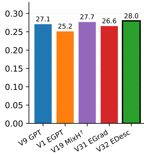
ARC-C
