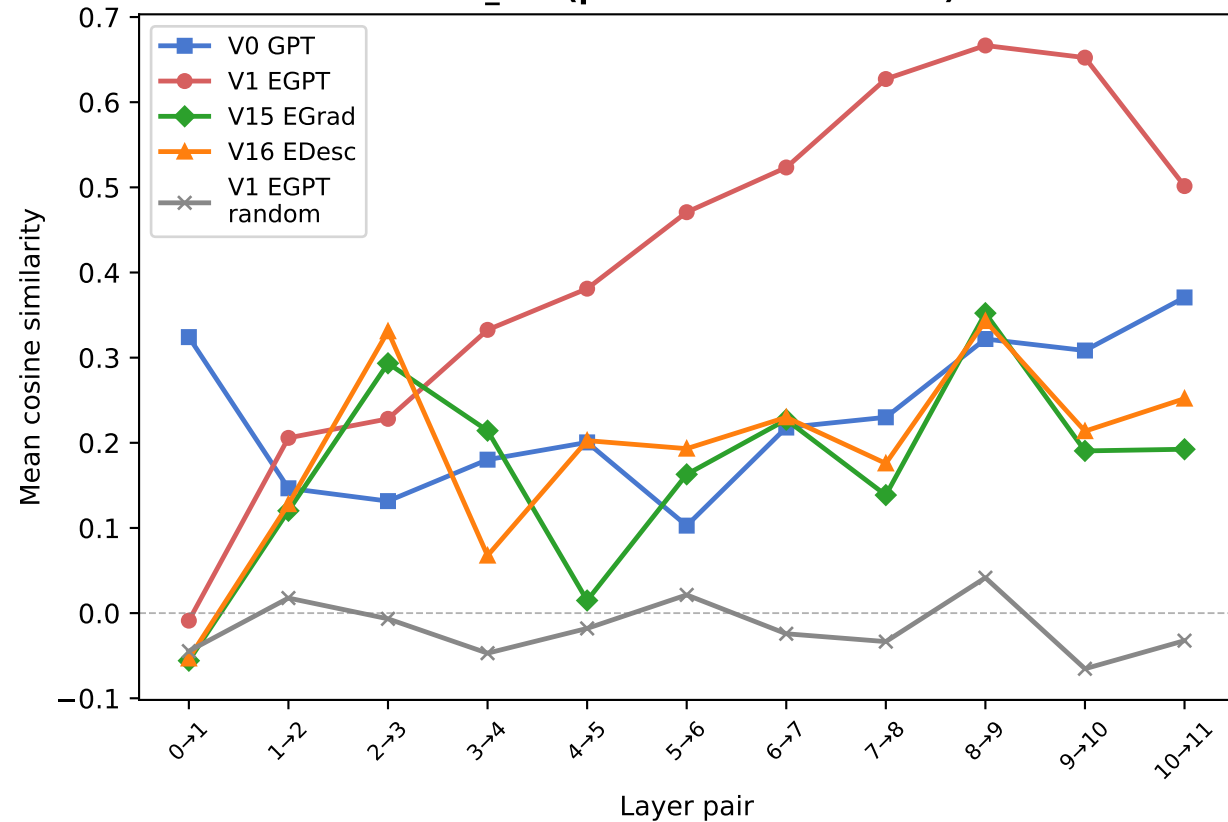
attn_out (pre-residual attention)
