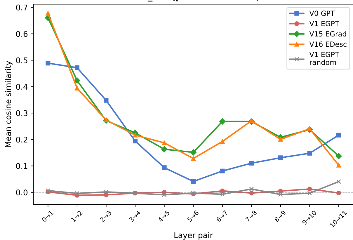
ffwd_out (pre-residual FFN)
