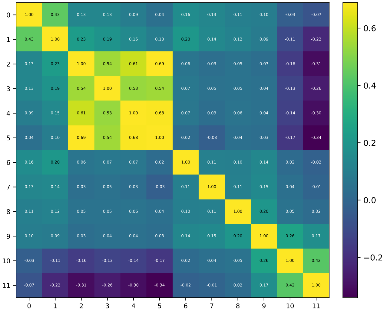
Block-Delta Cosine Sim — V0 GPT 12×1 d768
