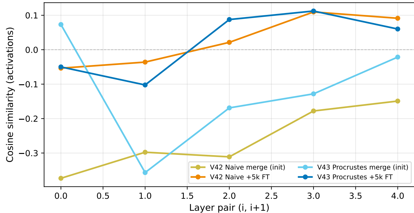
Block-Delta Cosine Sim, Consecutive Layers (6-layer merged)
