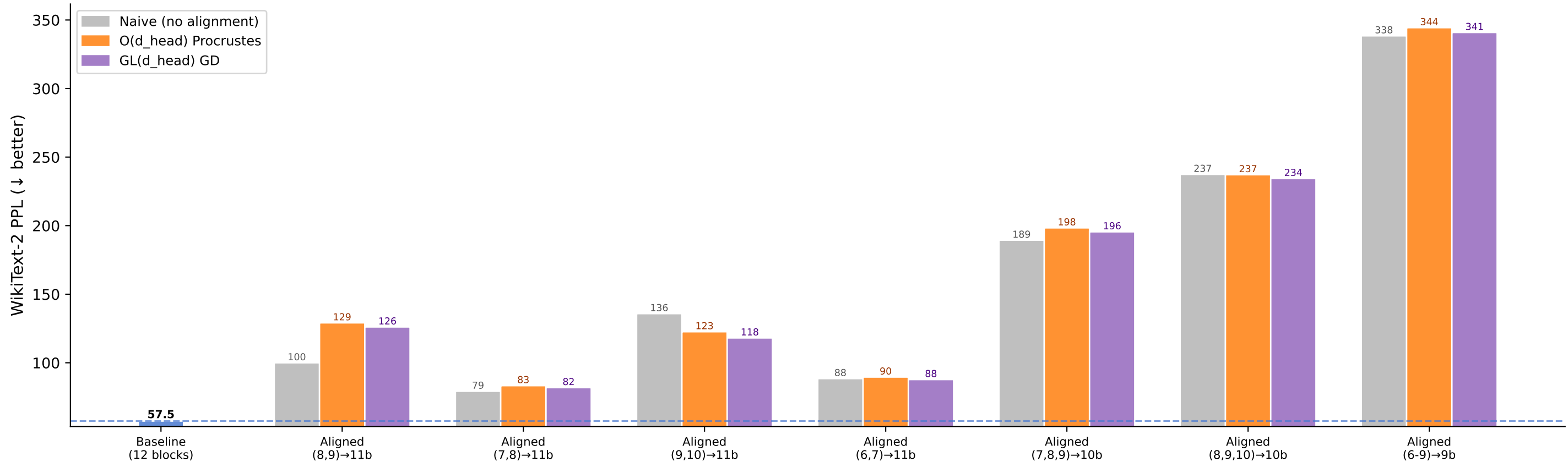
Layer-merge PPL: naive vs O(d_{\text{head}}) vs GL(d_{\text{head}}) alignment before averaging V1 EGPT \text{lr}=2\text{e-}3 | attn only (FFN kept), blocks dropped
