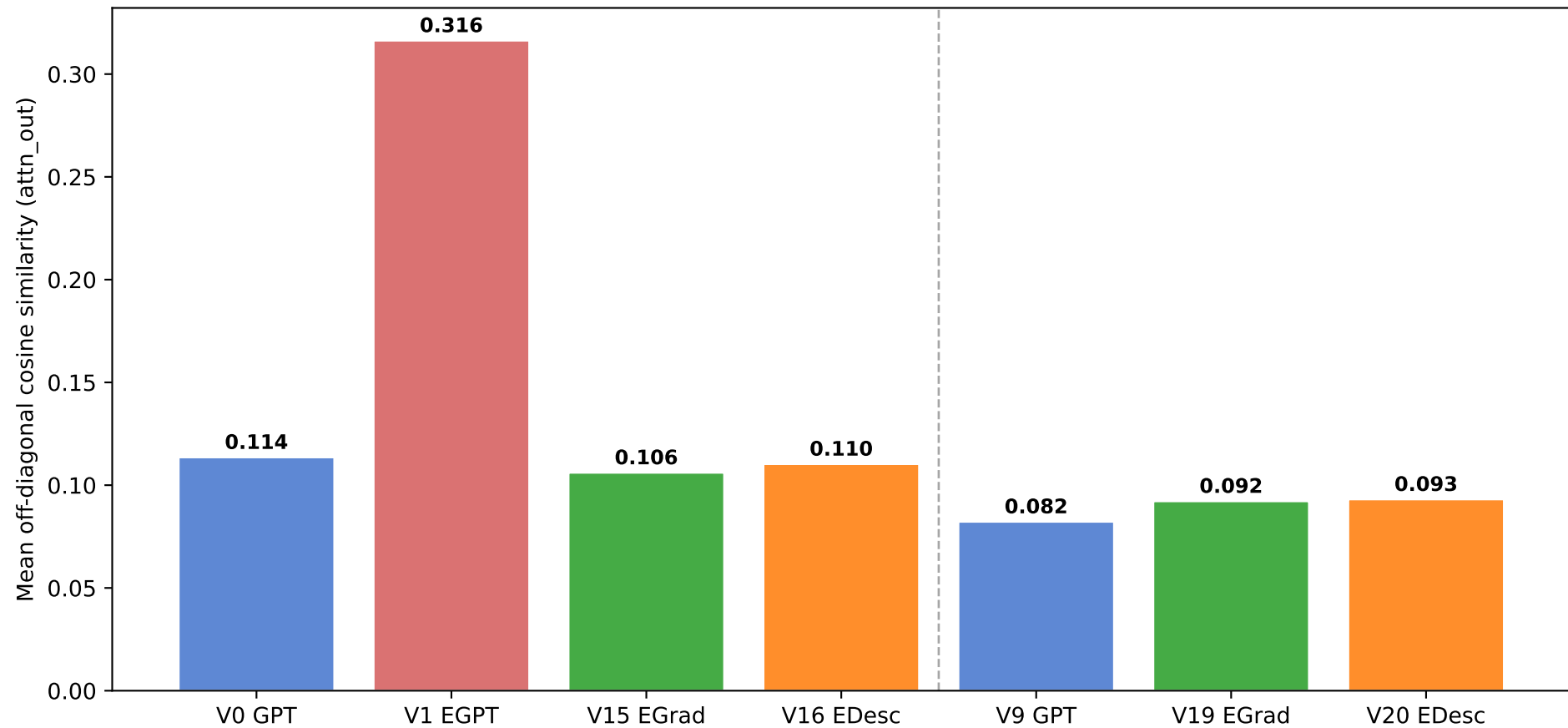
Inter-layer attention similarity: EGrad and EDesc vs baselines
