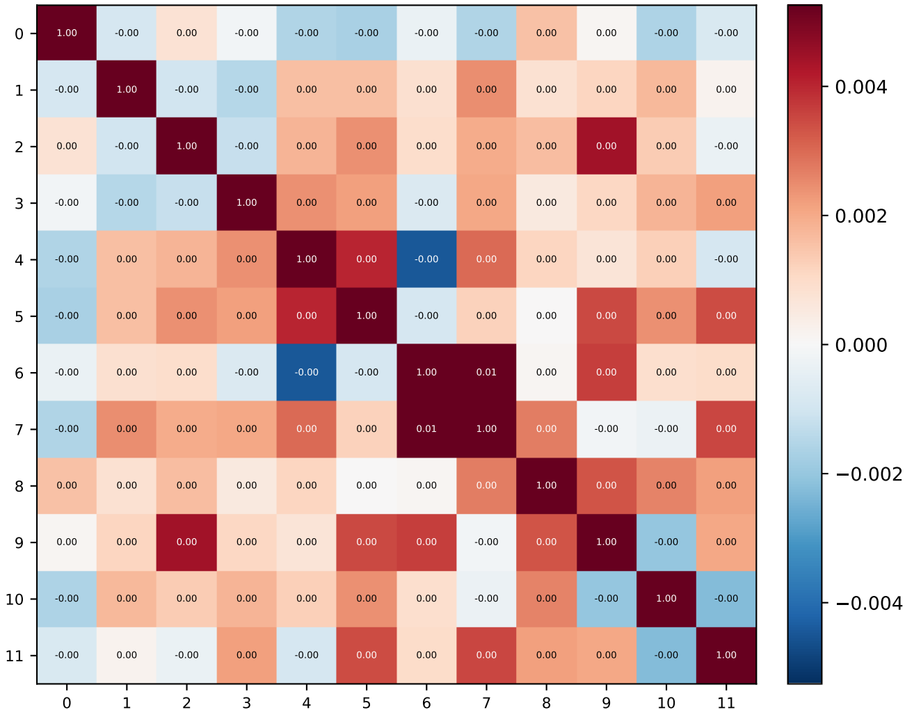
Attn Weight Cosine Sim — V1 EGPT 12×1 d768
