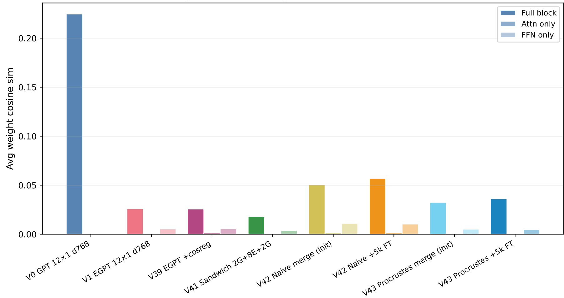
Avg Cosine Similarity: Full Block vs Attn vs FFN
