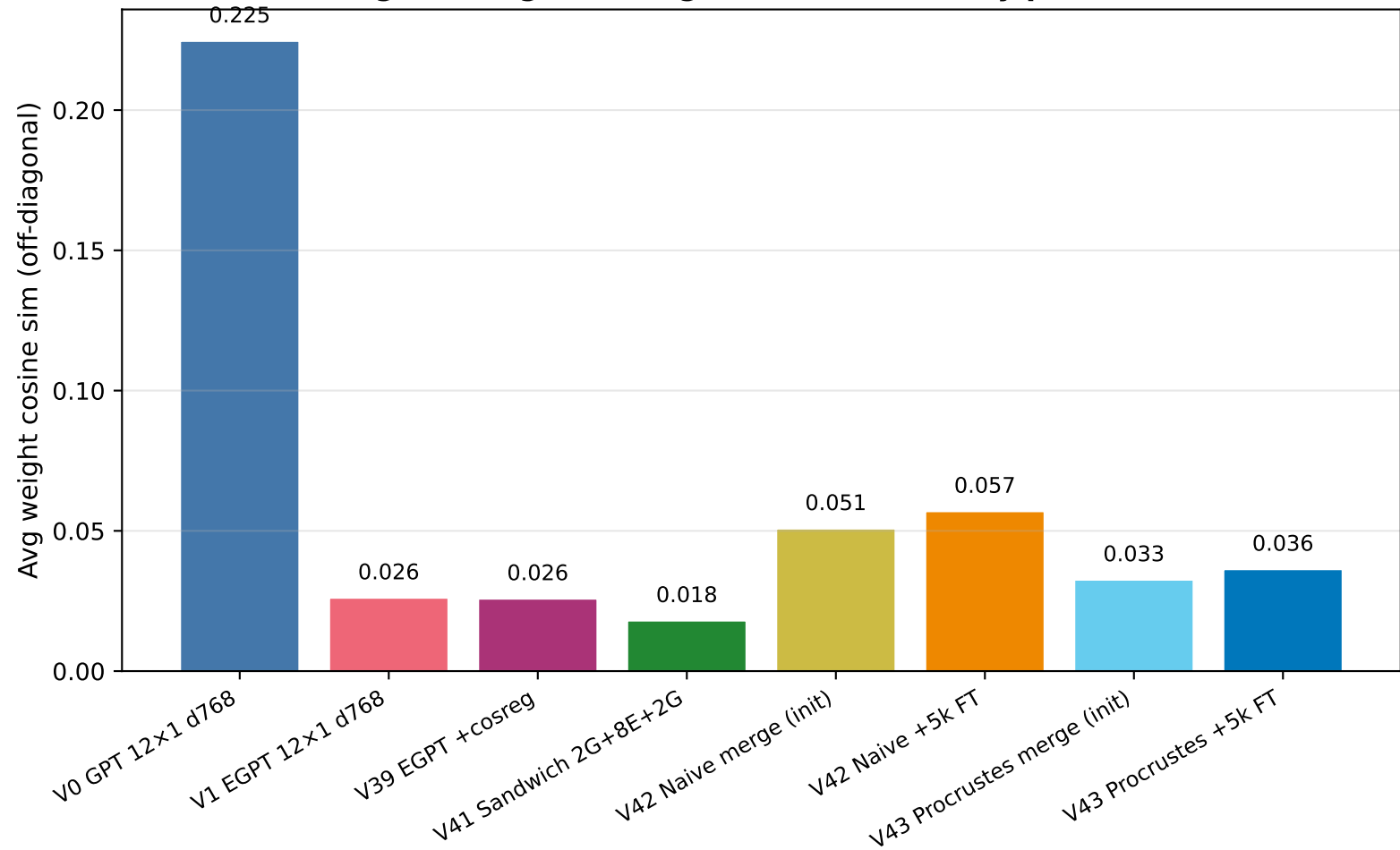
Avg Off-Diagonal Weight Cosine Similarity per Model
