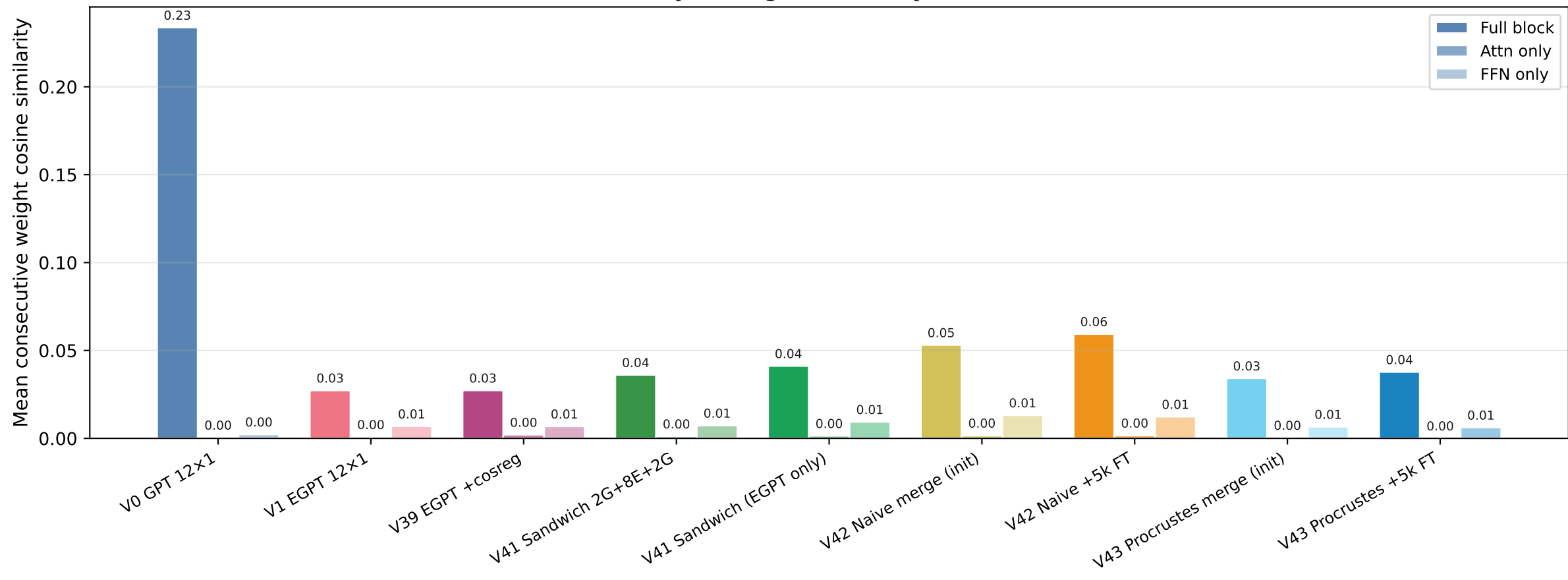
Consecutive-Layer Weight Similarity: Full vs Attn vs FFN
