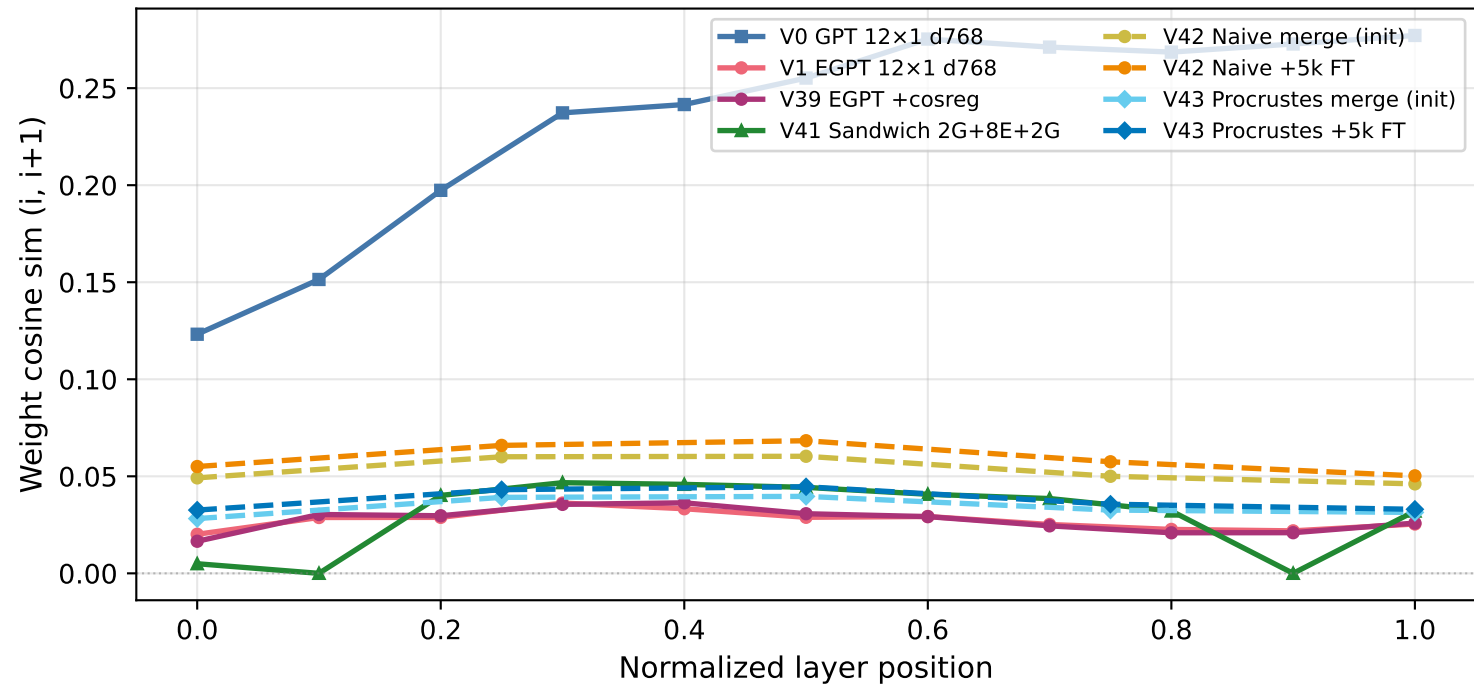
Consecutive-Layer Weight Similarity — All Merger Models
