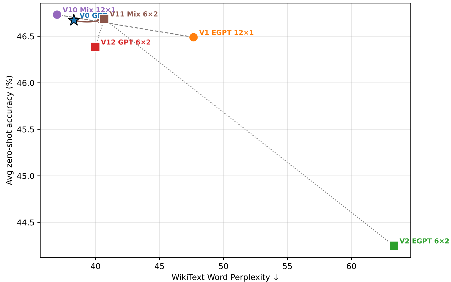
Accuracy vs Perplexity — all models ★=V0 baseline dashes=EGPT→Mixed within family
