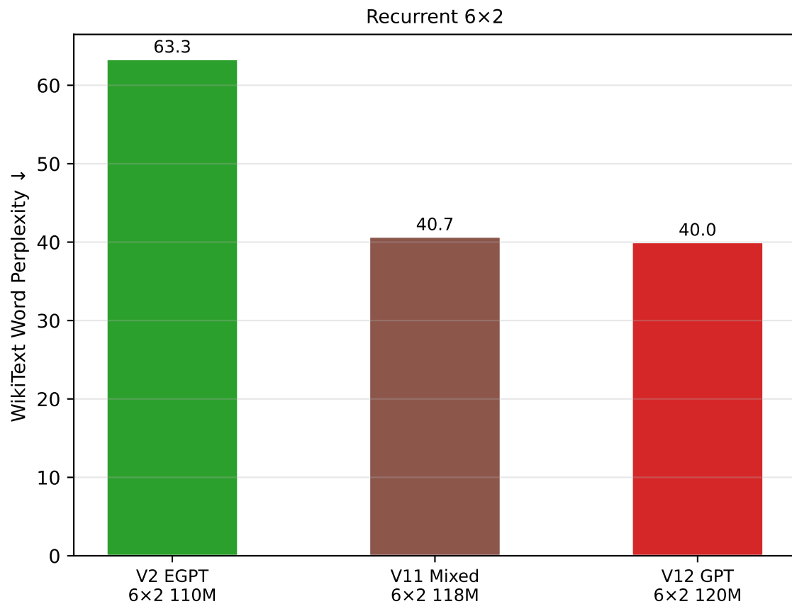
WikiText Perplexity: Mixed vs Pure Architectures (iso-family)
