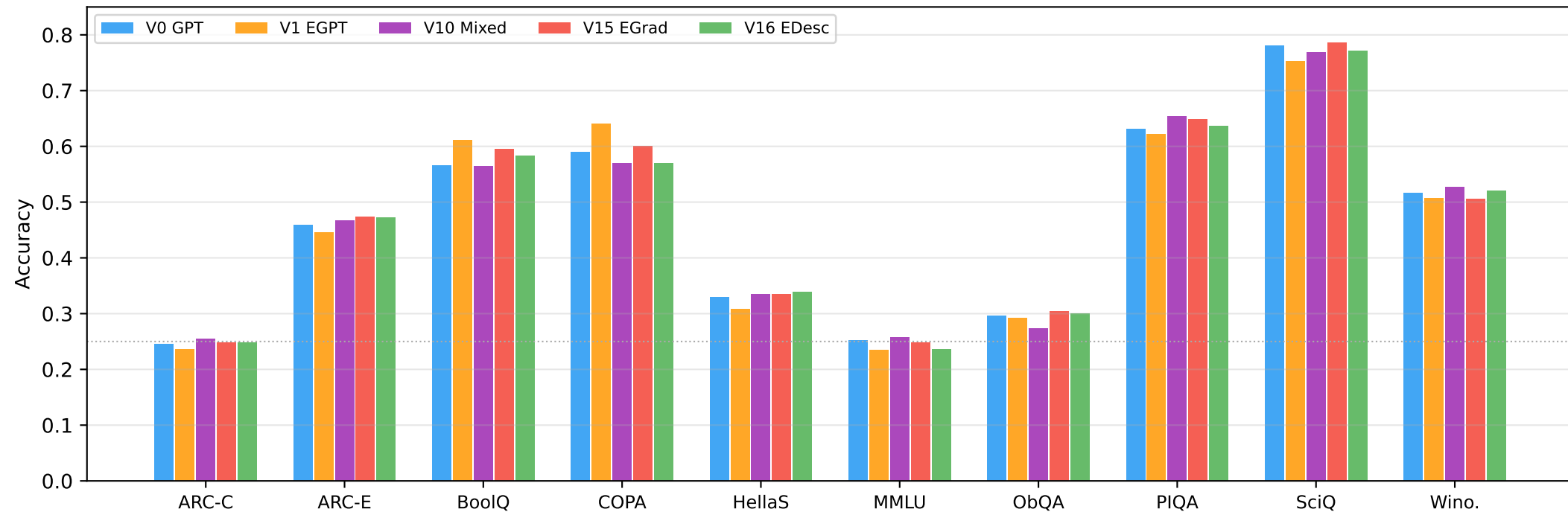
Output-rule ablation: V0 / V1 / V10 Mixed / V15 EGrad / V16 EDesc — per task
